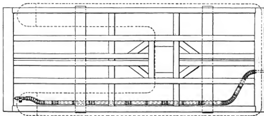
Fig. 3771. Arrangement of Steam Pipe Covering Under Tender.
